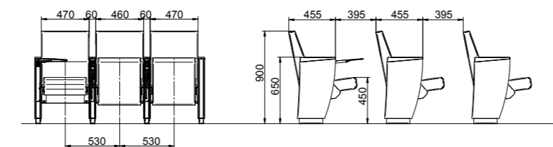
Aura Premium 500 with folding writing tablet
