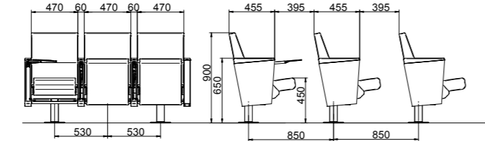
Aura Premium 500 with folding writing tablet
